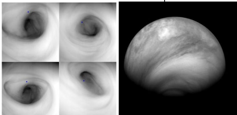
Figure 1 - l The polar region of Venus, at a wavelength of 3.8 microns, denotes the motion of the atmospheric vortex around a centre of rotation. The vortex center is found to be displaced on average by about 300 km from the South Pole (marked with a blue dot) and rotating around it in an unexplained precession movement (ESA/VIRTIS-VenusX/INAF-IASF/LESIA-Obs. Paris).
