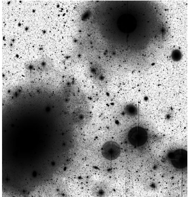
Figure 4 - Elixir-LSB image of the NGVS-1-4 pointing in g' , including Messier 49 in its lower left corner. The large object at the top results from a very bright star ( V=6 ) reflections in the optics. The fainter features seen on this image (e.g. shells) reach the 29th magnitude per square arcsecond.
