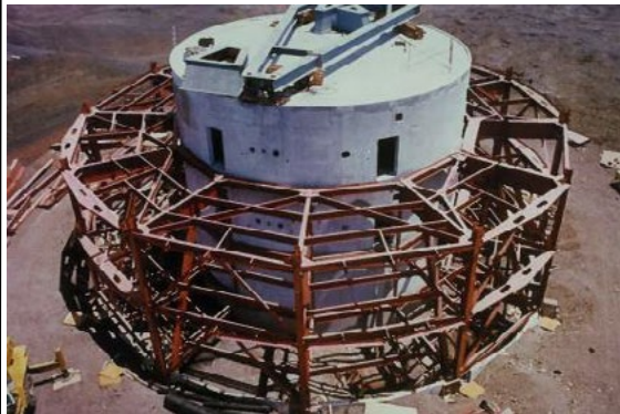
The pier is seen during construction with the base (A-frame) of the telescope already installed at its top. The metallic structure being erected around will ultimately support the dome.
